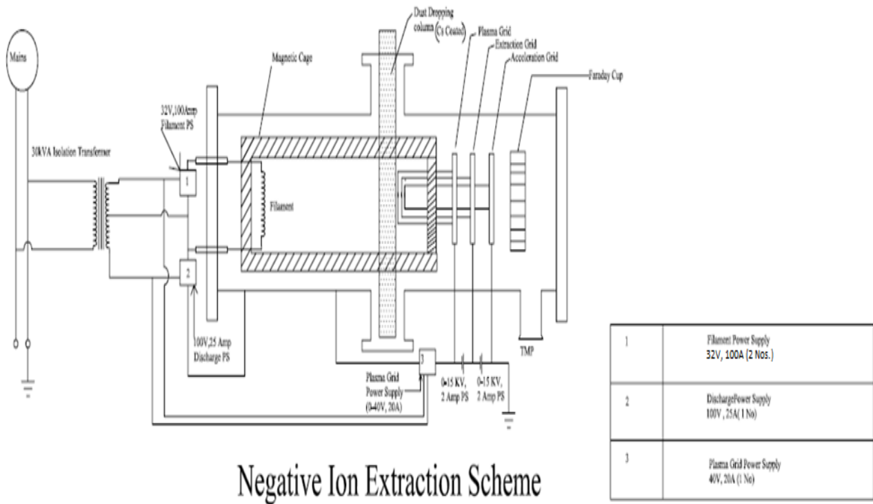
Fig. 2: Schematic diagram of the negative ions extraction scheme
