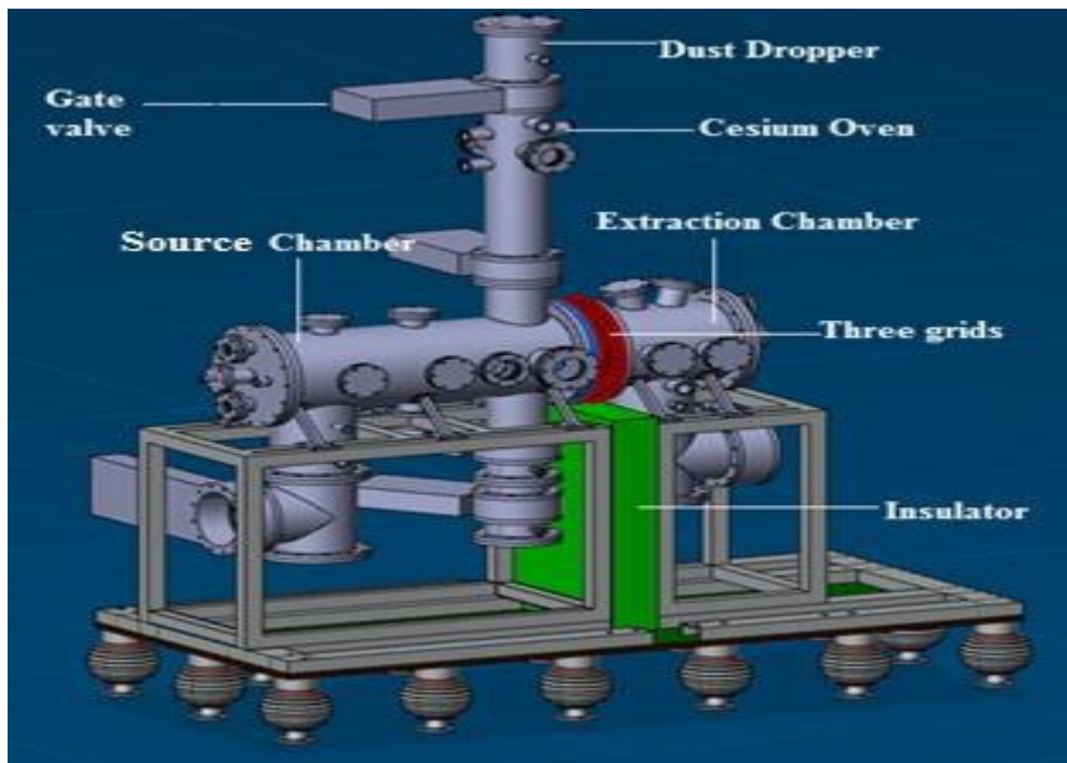
Fig. 1: View of the experimental setup
