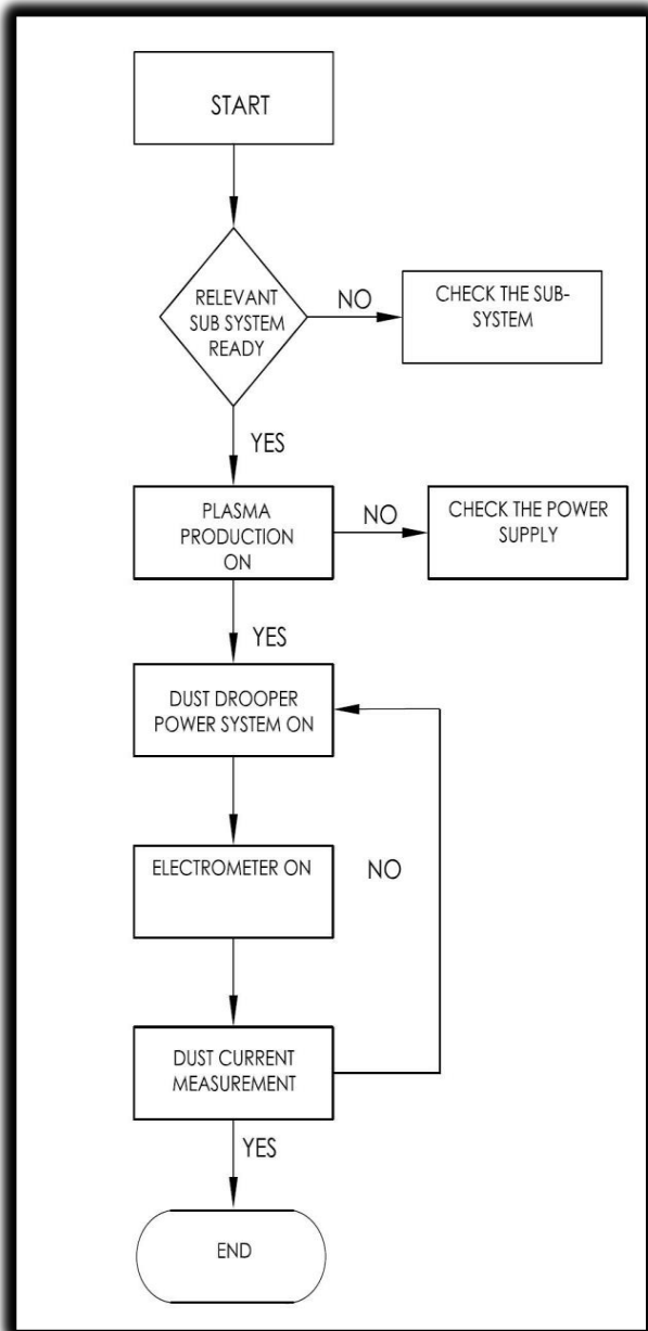
FLOW CHART FOR MEASURING PLASMA PARAMETERS USING LP WITHOUT CS
